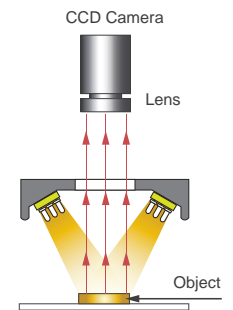
Illumination structure
