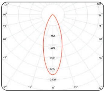
Illumination Diagrams
