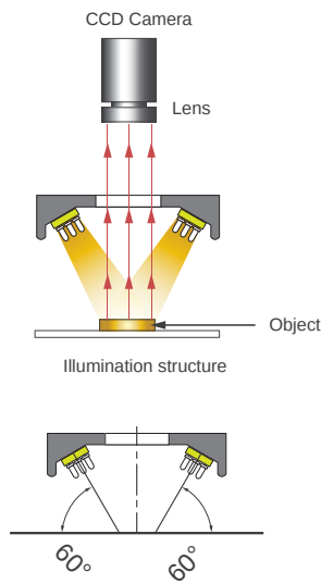
CIR series angle diagram (*1 The angle between light and horizontal)
